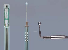
Expanded Seven Air Velocity Probe Line-up
